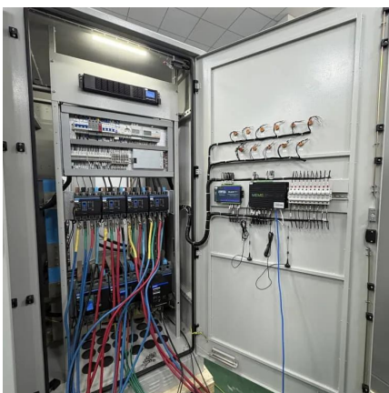
ENERGY STORAGE CHARGING PILE INSTALLATION IN KUWAIT CITY
